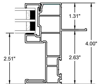
Horizontal Section through Picture Window
