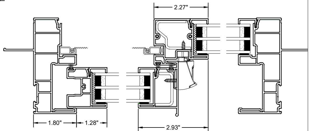
Horizontal Section through Slider
