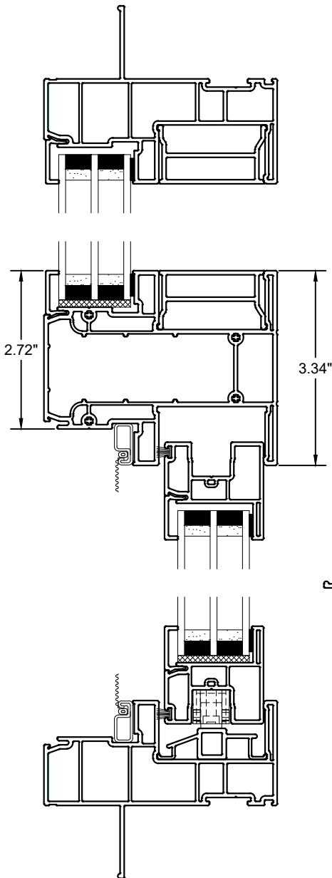
Vertical Section
