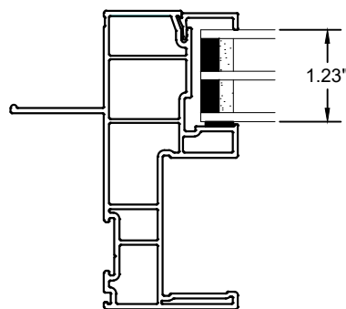
Horizontal Section through Picture Window
