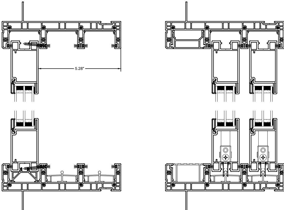
Vertical Section through Fixed Lite
