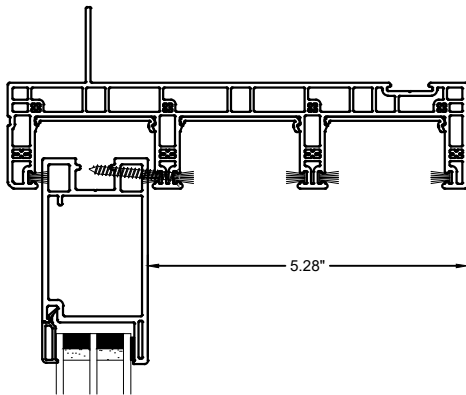
Vertical Section through Fixed Lite
