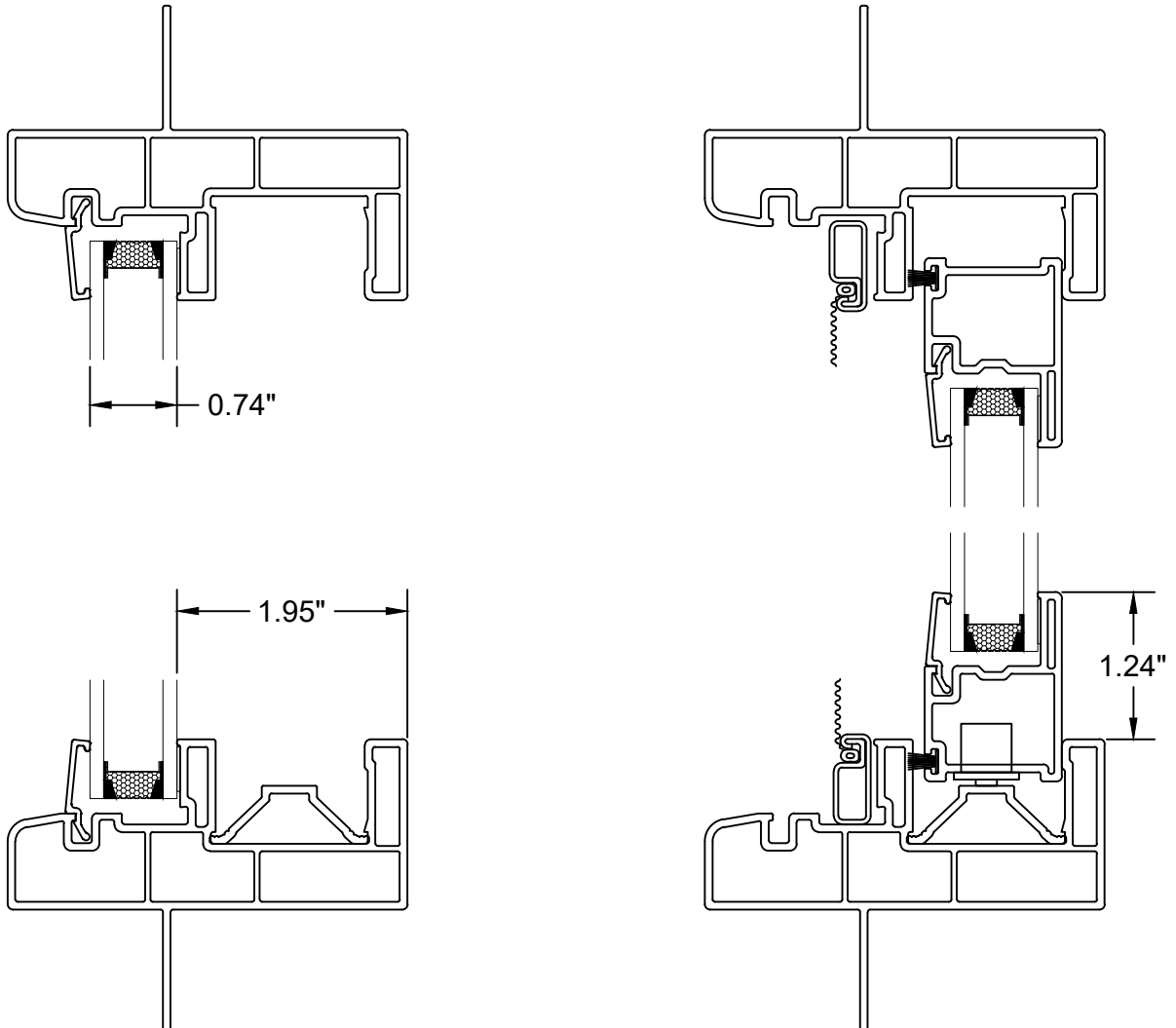
Vertical Section through Fixed Lite
