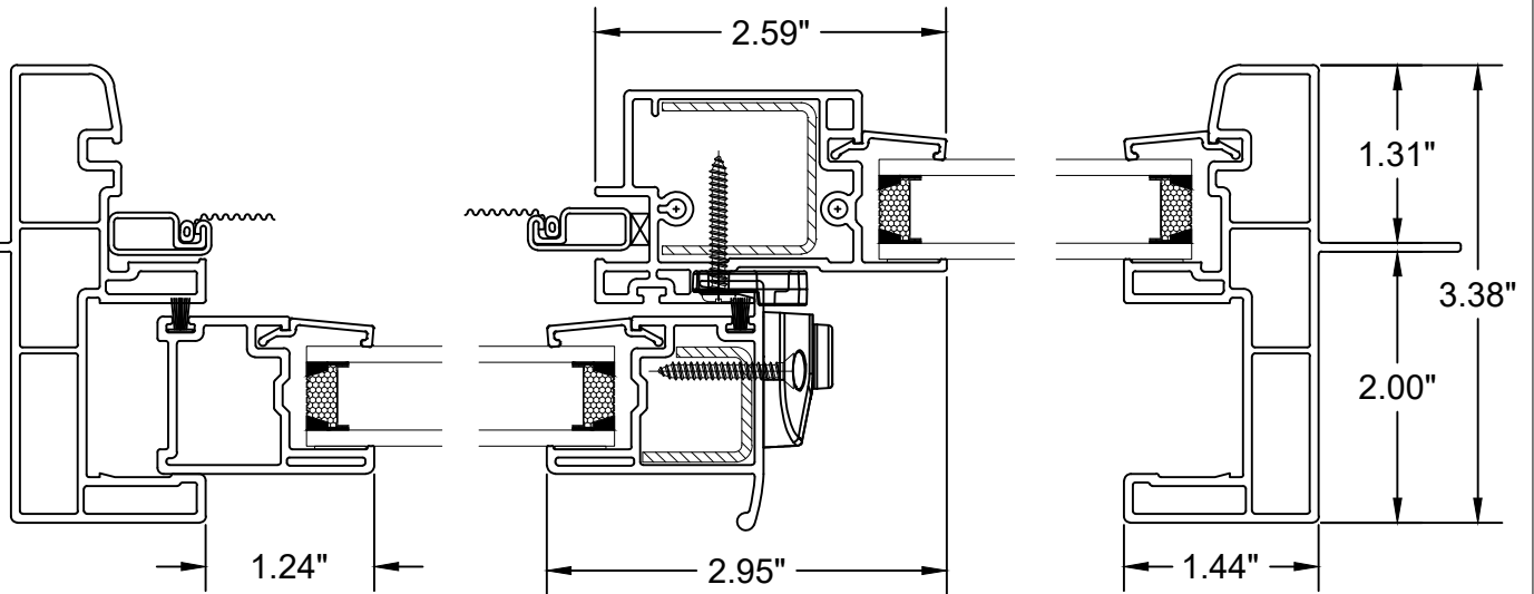
Horizontal Section
