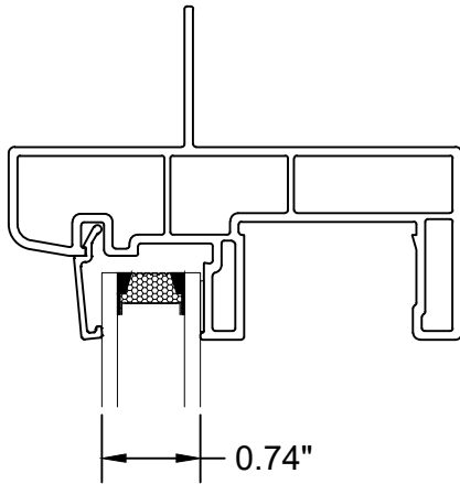
Vertical Section through Fixed Lite
