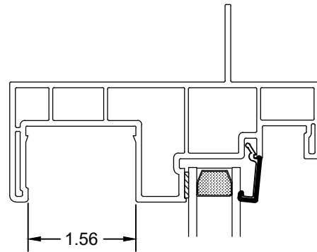
Vertical Section through Fixed Lite
