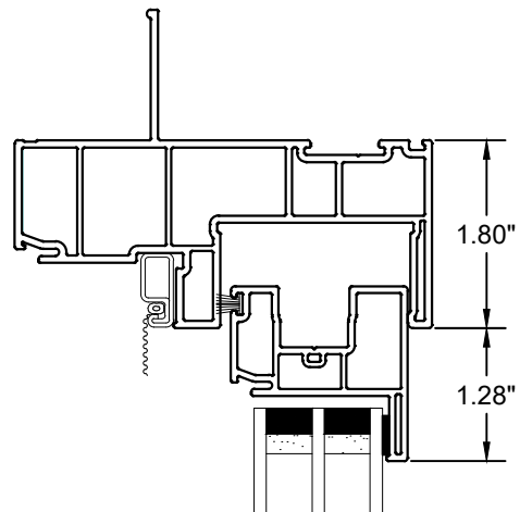
Vertical Section through Sash
