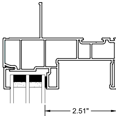
Vertical Section through Fixed Lite
