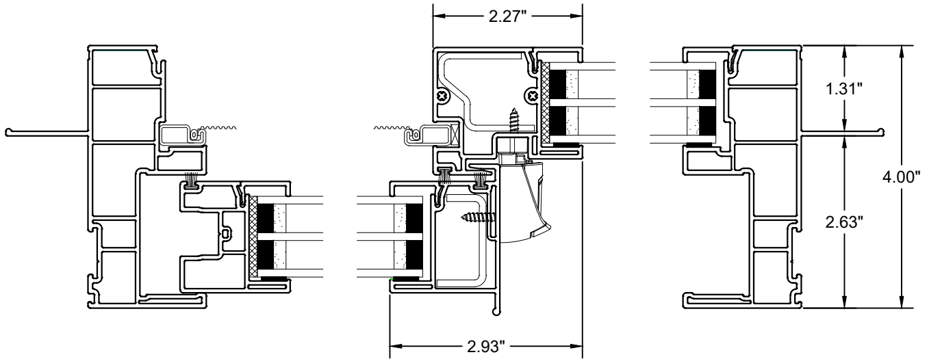
Horizontal Section
