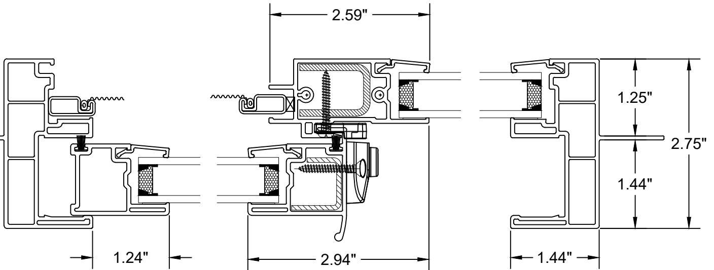
Horizontal Section
