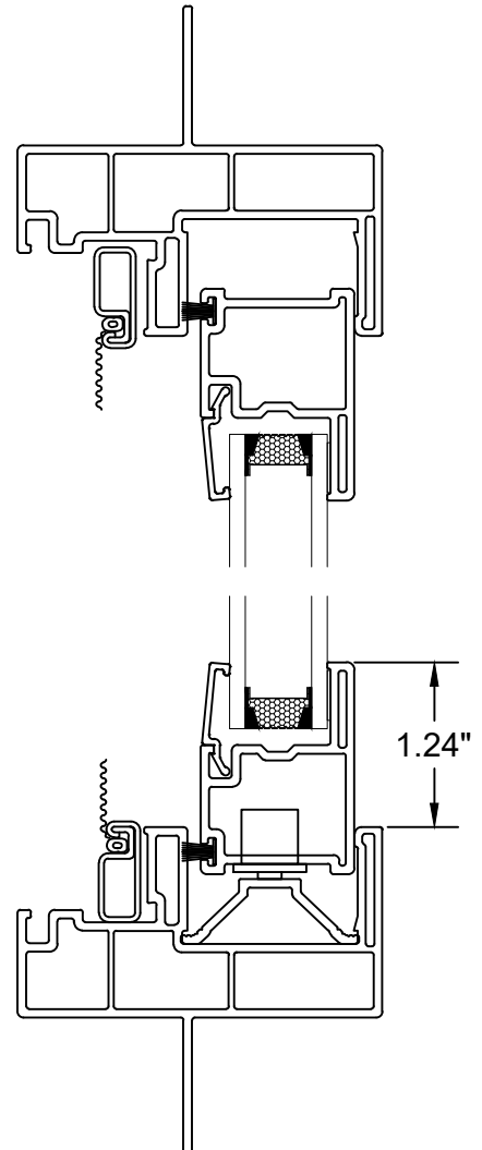
Vertical Section through Sash
