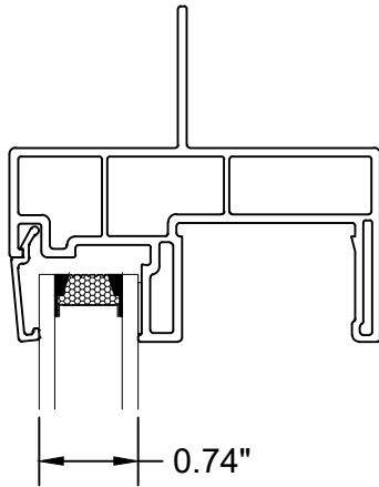
Vertical Section through Fixed Lite
