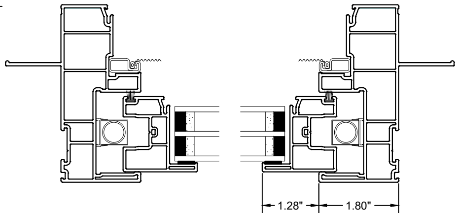
Horizontal Section through Sash
