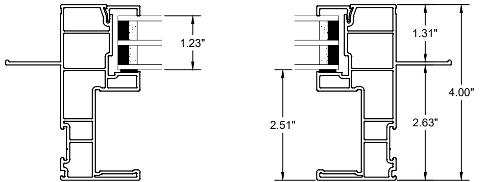
Horizontal Section through Fixed Lite
