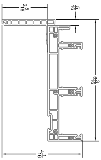
6000 Series 2 Track Door Frame (w/ Flush Fin)
