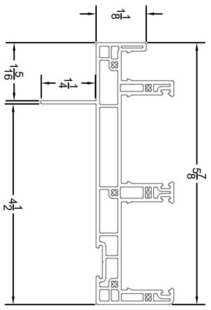
6000 Series 2 Track Door Frame
