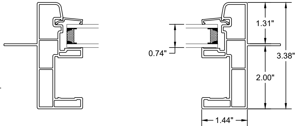
Horizontal Section through Fixed Lite
