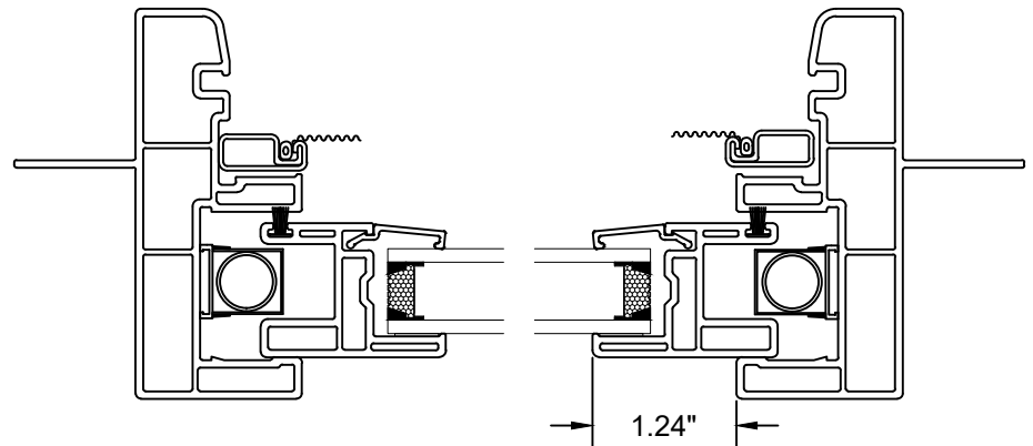
Horizontal Section through Sash
