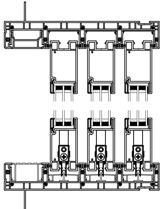
Vertical Section through Sashes
