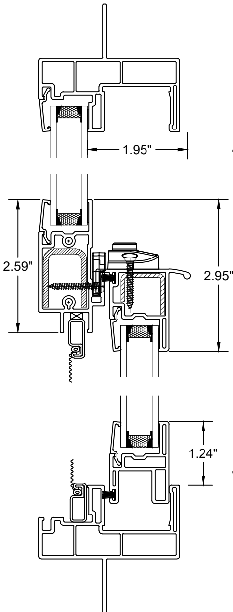
Vertical Section
