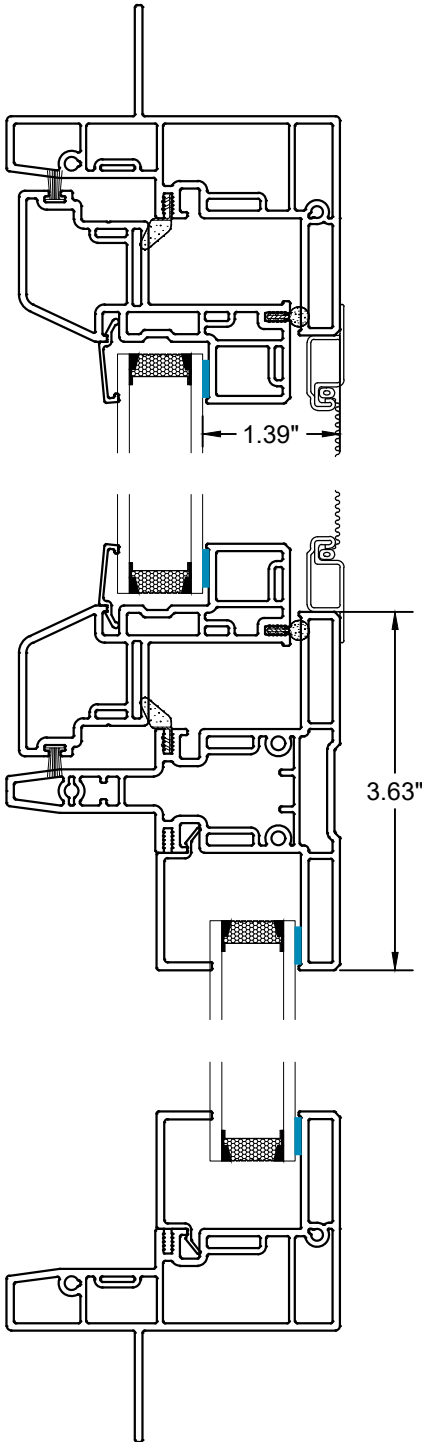
Vertical Section
