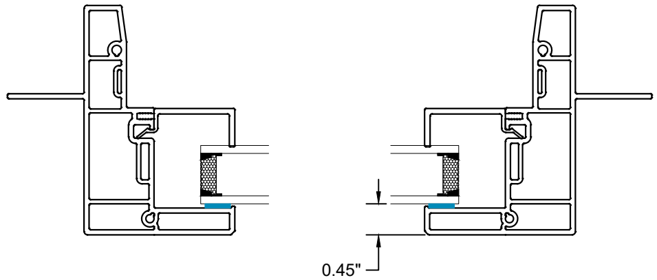
Horizontal Section through Fixed Lite
