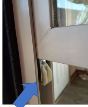
The balancer shoe should now be somewhat exposed
