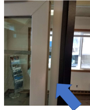
Push the sash in against one jamb allowing clearance for the other side
